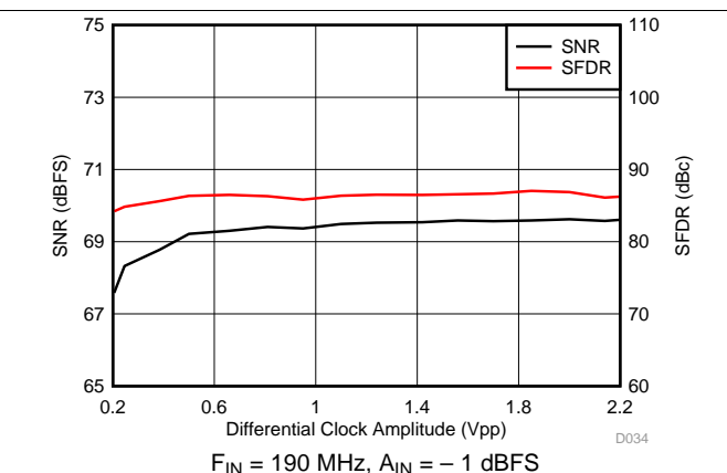
Figure 35. Performance vs Clock Amplitude
