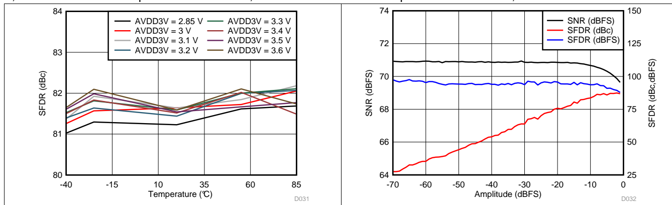
Figure 32. Spurious-Free Dynamic Range vs AVDD3V Supply and Temperature
