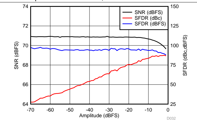
Figure 33. Performance vs Amplitude
